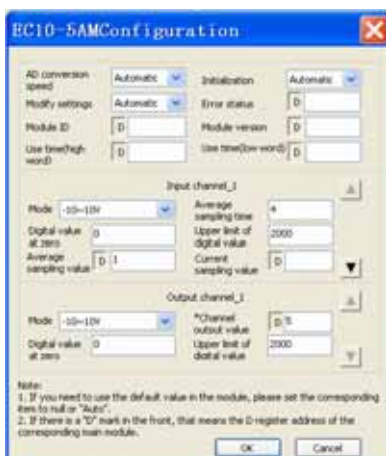
Figure 4-2 Setting special module parameters
