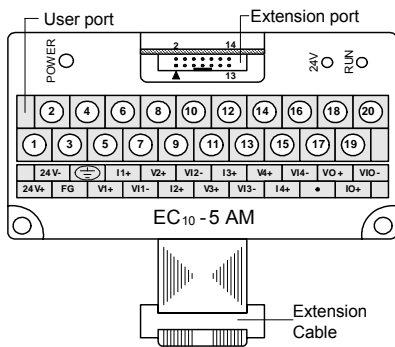
Figure 1-2 Extension port and user port
