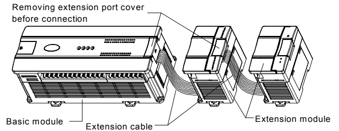
Figure 1-3 Connecting EC10-5AM to the basic module
