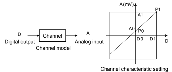
Figure 3-4 EC10-5AM output channel characteristic
