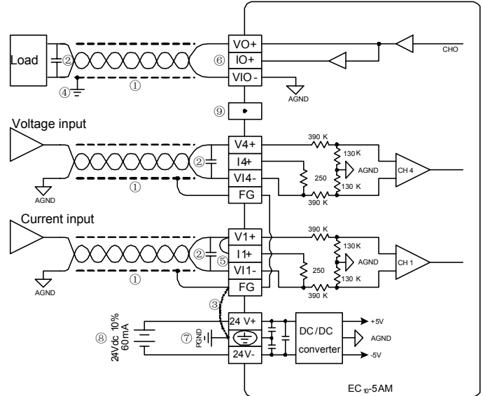
Figure 1-4 Wiring of EC10-5AM user port
