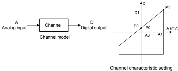
Figure 3-1 EC10-5AM input channel characteristic
