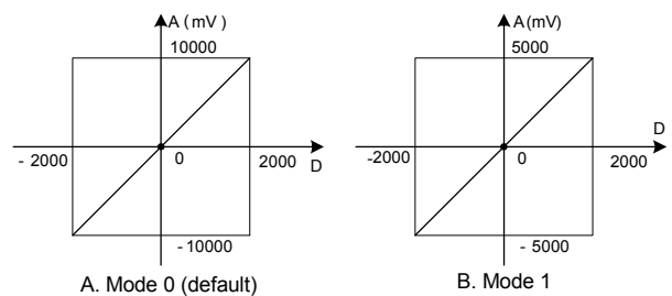
Figure 3-5 Default output channel characteristics in various modes
